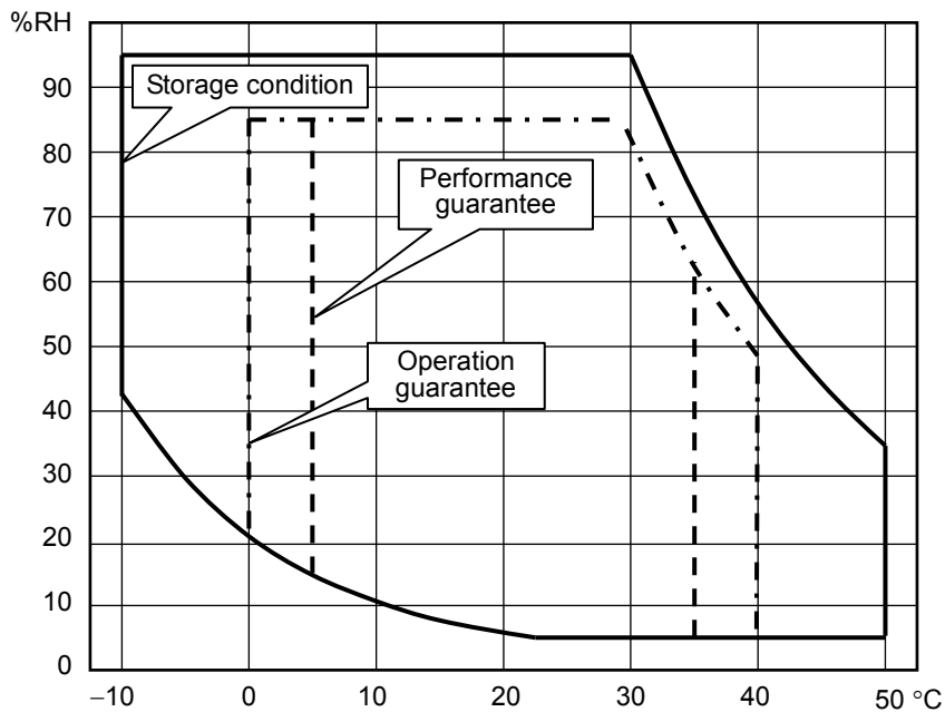
Figure 1-1. Temperature and Humidity Ranges
